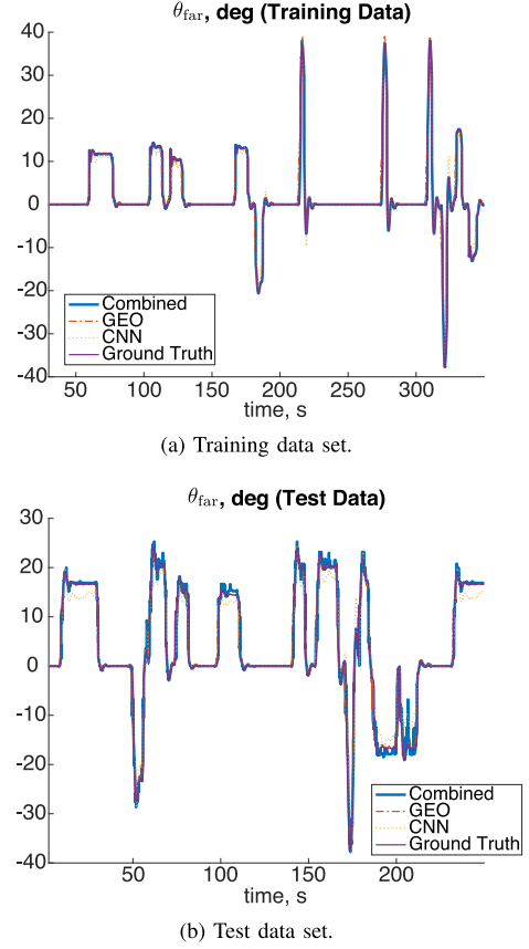
Fig. 10. The results of \theta_{\text{far}} estimations.
