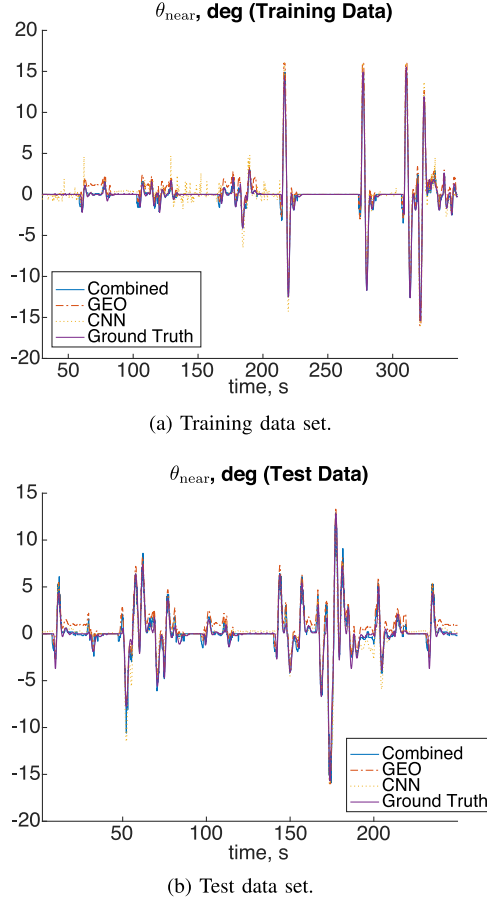
Fig. 9. The results of \theta_{\text{near}} estimations.
