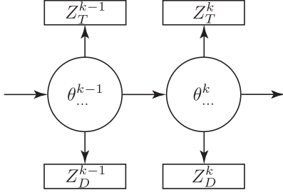
Fig. 6. The structure of the proposed DBN.
