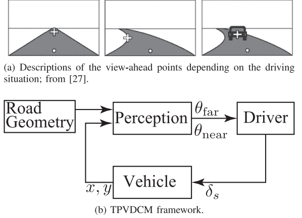
Fig. 2. Two-point visual driver control model.
