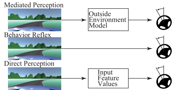
Fig. 1. Comparison of self-driving vehicle control approaches.
