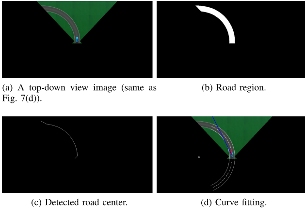
Fig. 8. The process of detecting the view-ahead angles from the top-down view image Fig. 7(d).
