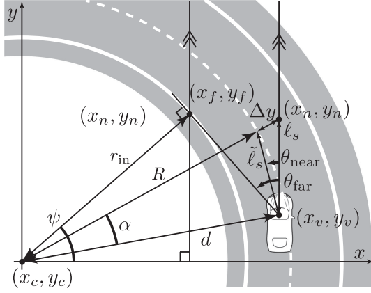
Fig. 4. Illustration of \theta_{\text{far}} and \theta_{\text{near}} when the road is curved.
