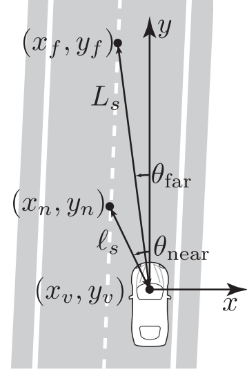
Fig. 5. Illustration of \theta_{\text{far}} and \theta_{\text{near}} when the road is straight.
