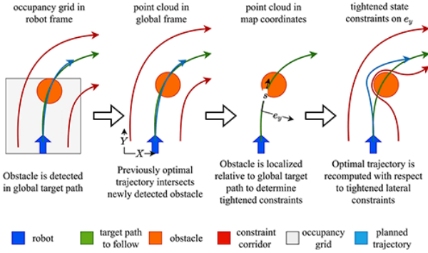
Fig. 9: Obstacle avoidance pipeline.
