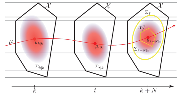
Fig. 1: A schematic describing the proposed CS-SMPC approach.
