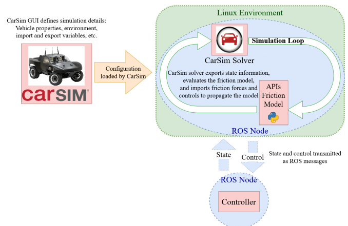
Fig. 3: AutoRally simulation environment.
