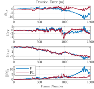
Figure 2. Position error (m) in LVLH. Rows 1-3 indicate the across track, cross track, and radial directions, while row 4 shows the error norm.
