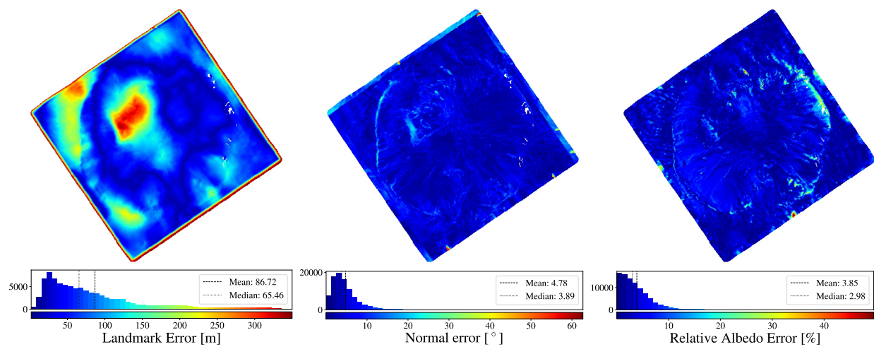
Figure 3. Quantitative comparison between our solution and the SPC baseline with respect to landmark error, normal error, and relative albedo error.
