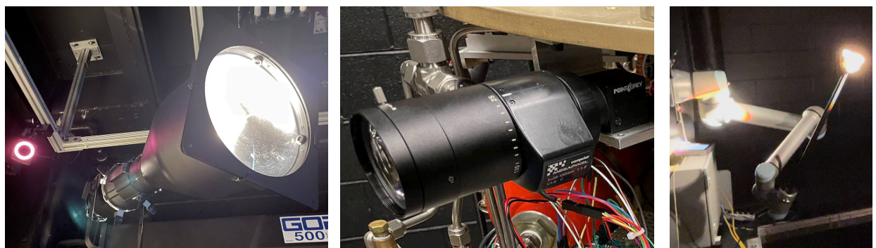
(d) Collimated-Beam Light Source and VICON Motion Capture System (e) Small FOV camera optics (f) RMS and mock asteroid
