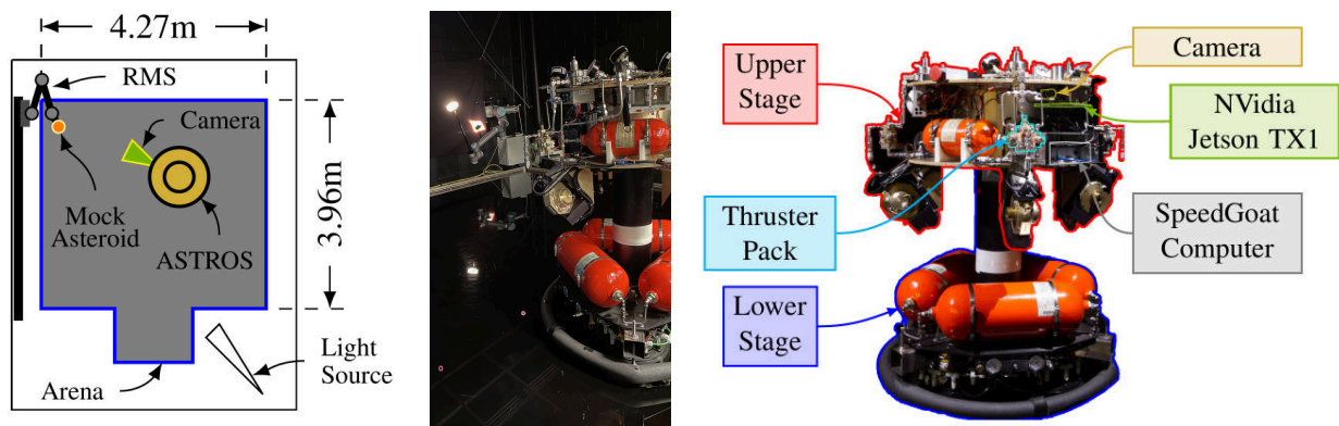
(a) Disposition of Devices in (b) ASTROS in Arena (c) Main Components of ASTROS Test Bed Arena
