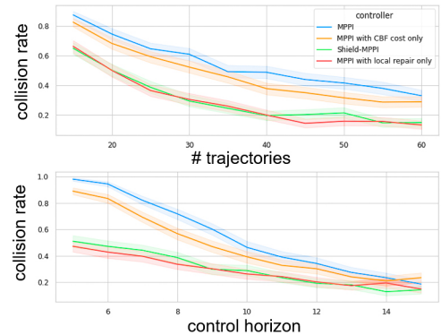
Fig. 5: Comparison of MPPI and Shield-MPPI using CPU implementation.
