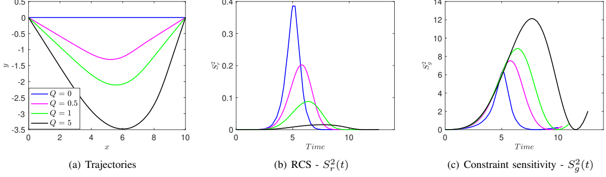
Fig. 2. Results for constraint desensitized 2D path planning
