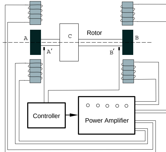
Figure 1: Magnetic bearing/rotor system.
