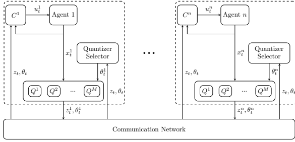
Fig. 1. The n agent model with all-to-all communication framework.
