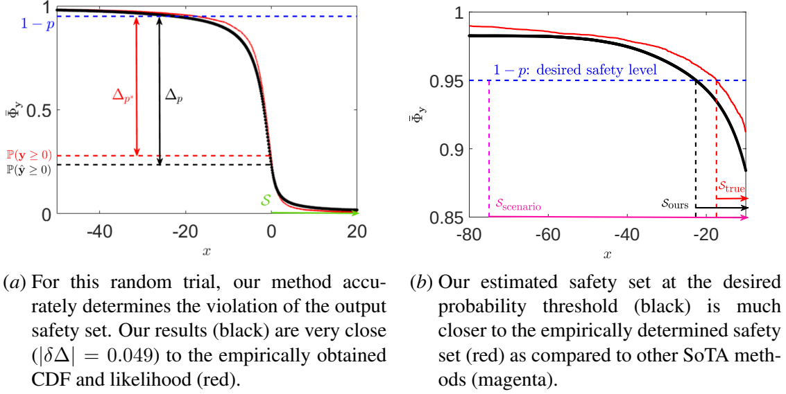
Figure 3: Comparison of ReLU network safety verification.
