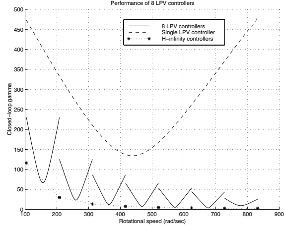
Figure 9: Performance of narrow band LPV controllers.
