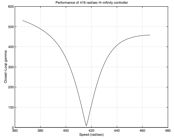
Figure 3: Single speed \mathcal{H}_\infty controller operated over a range of speeds.
