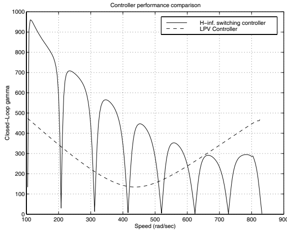
Figure 8: \mathcal{H}_\infty and LPV controller performance.
