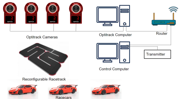
Fig. 1. BuzzRacer system components.
