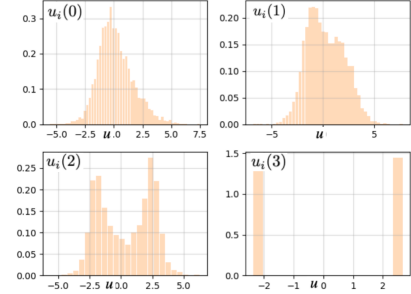
Fig. 5. The histograms of u_i(k) at time step k for each agent i . The upper left and right figures are u_i(0) and u_i(1) , i = 1, \dots, 5000 respectively. The lower left and right figures are u_i(2) and u_i(3) respectively.
