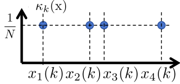
Fig. 1. An illustration of the probability distribution \kappa_k(x) of group system state x(k) . Each x_i(k) is a sample from \chi_k(x) in \kappa_k(x) .
