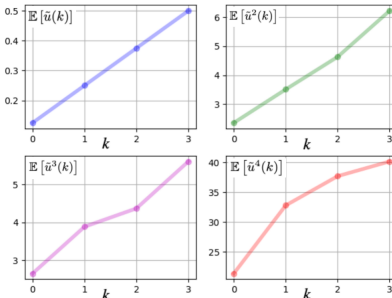
Fig. 3. \tilde{u}(k) at time steps k = 0, 1, 2, 3 .
