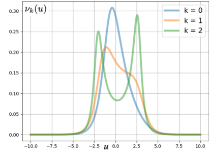
Fig. 4. Realized distributions of control inputs \nu_k(u) by \tilde{u}(k) for k = 0, 1, 2 , which are obtained by our proposed control scheme.
