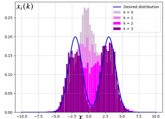
Fig. 6. The histogram of the terminal distribution of x_i(k) , i = 1, \dots, 5000 compared to the desired distribution. It is close to the specified terminal distribution (27).
