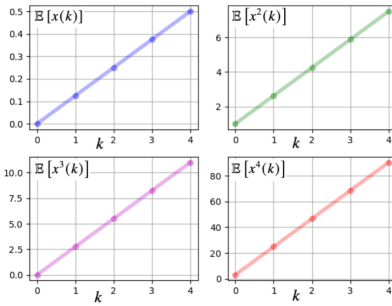
Fig. 2. \mathcal{X}(k) at time steps k = 0, 1, 2, 3, 4 .
