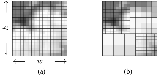
Fig. 1: (a) Full resolution occupancy grid; (b) Compressed (i.e., quantized) occupancy grid.
