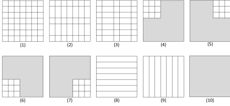
Fig. 6: Set of Abstractions used for the simulations. The grey area denotes no information about these cells
