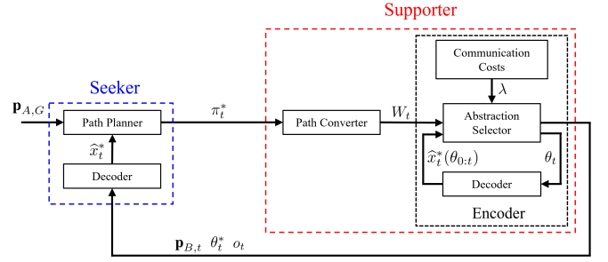
Fig. 2: Flowchart that presents the proposed framework's architecture at timestep t . The Seeker shares its current optimal path \pi_t^* to the Supporter. The Supporter utilizes this to select the optimal abstraction of its local map \theta_t^* \in \Theta and sends it to the Seeker to aid in reaching its target.
