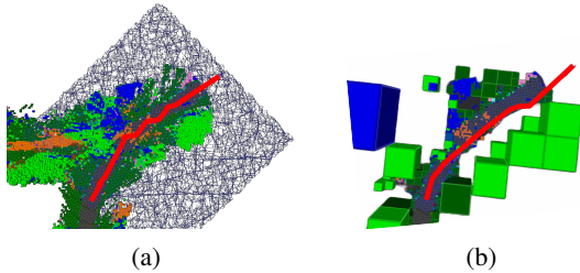
Fig. 6: (a) The optimal path found by COA* in the graph constructed with a Halton sequence. (b) The optimal path found by COA* in the graph constructed based on the compressed octomap nodes.
