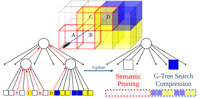
Fig. 1: Semantic octree update from a new observation indicating cell D is blue and C is free space. Each leaf node with color-encoded object class is depicted as a square, inner nodes are represented by circles, and unexplored cells are shown as dots. Multi-class probabilities and G-values along the paths from leaf nodes to the root, highlighted in red, need to be updated due to the new perceptual data.
