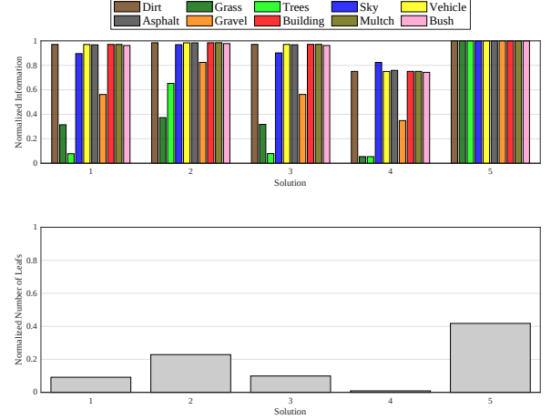
Fig. 4: (top) Normalized degree of information retained for each semantic class as a function of the G-tree search weights (solution number). (bottom) Normalized number of leaf nodes of the compressed octree.
