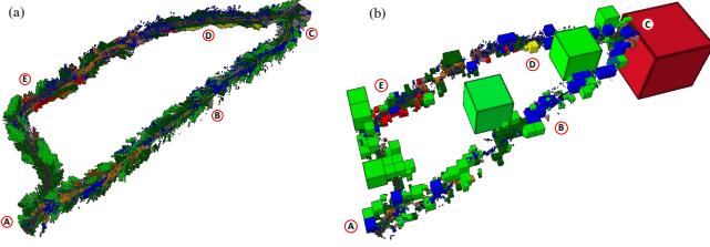
Fig. 3: (a) finest-resolution semantic octree representation build from point-cloud data. (b) Compressed multi-resolution octree obtained from the framework in Section III.
