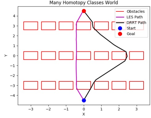
Fig. 2: Planning with the proposed LES-RRT # and DRRT [28] in a world with multiple homotopy classes. The computationally costlier DRRT (black path) can get “stuck” in a wrong homotopy class. For the above trial run, LES-RRT # and DRRT sampled 9414 and 573 graph vertices respectively in 1 second of planning time.
