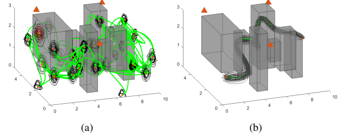
Fig. 5: Planning results of the 3-D double integrator
