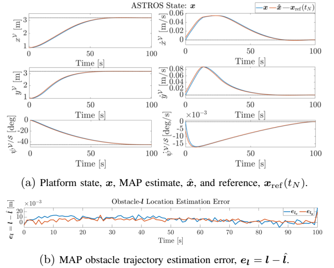
Fig. 13: Predictive SCATE simulation trajectories and estimations.
