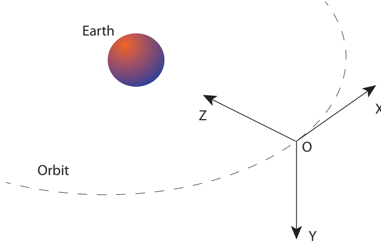
Figure 4. The local-vertical/local-horizontal (LVLH) reference frame used in most attitude control problems for spacecraft in orbit. The origin O of the LVLH frame is located at the center of mass of the spacecraft and follows it as it goes around the orbit.
