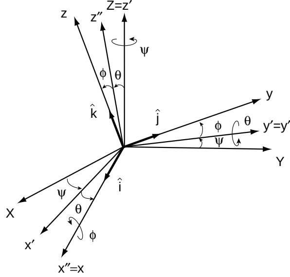
Figure 2. Euler angle sequence (3-2-1). We align the inertial and body frames by first rotating with an angle \psi about the z -axis, then rotating with an angle \theta about the new y -axis, and finally rotating with an angle \phi about the x -axis.
