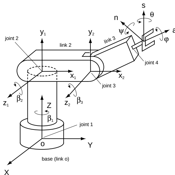
Figure 7. Typical robotic manipulator consisting only of revolute joints. The attitude of the gripper is given by the orientation of the (a, s, n) body frame. The geometry of the manipulator determines the orientation of this frame with respect the joint angles \beta_1, \beta_2 and \beta_3 .
