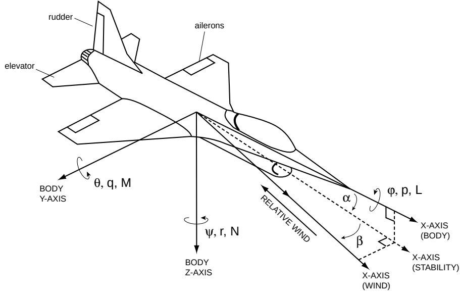
Figure 6. Body reference frames on an airplane. The stability axes differ from the wind axes by the sideslip angle \beta , and the body-fixed axes differ from the stability axes by the angle of attack \alpha . The angles \alpha and \beta change as the relative velocity of the airplane to the wind changes.
