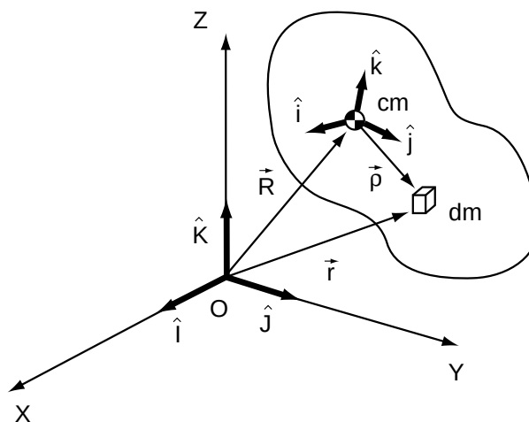
Figure 1. Inertial and body-fixed reference frames. The body-fixed reference frame is located at the center of mass cm . The vector \vec{r} denotes the location of the element mass dm in the inertial frame and the vector \vec{p} denotes the location of the mass in the body frame.
