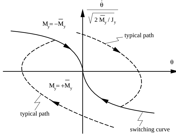
Figure 5. Bang-bang minimum time control of a single-axis attitude maneuver. If the initial orientation and velocity of the body is below the switching curve, the control logic will switch from the maximum to the minimum possible torque. The opposite if true is the initial condition is above the switching curve.
