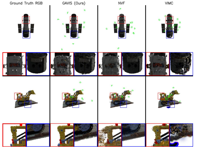
Figure 5. Qualitative active mapping. Reconstruction results and camera-view distributions (green frustums) from different methods’ active-mapping trajectories on HST scene (top) and Lego scene (bottom). Full results are provided in Sec. 12.
