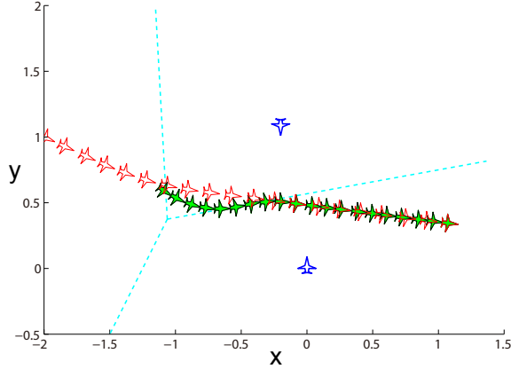
Fig. 5. Trajectory of the active pursuer (in red) and optimal trajectory of the evader (in green) obtained from GPOPS. The cyan line represents the Voronoi diagram of the three pursuers with initial conditions.
