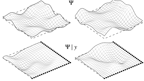
(b) Two-dimensional GRF \Psi conditioned to have the rightmost edges be constant
