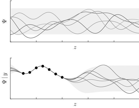
(a) Single-dimensional GRF \Psi conditioned on measurements
