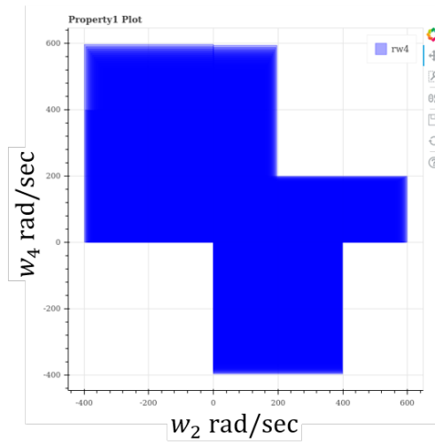
(c) C2E2
