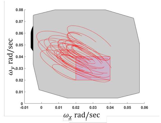
(b) CORA
