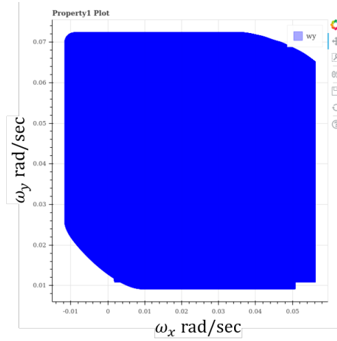
(c) C2E2
