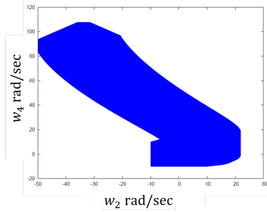
(a) Flow*
