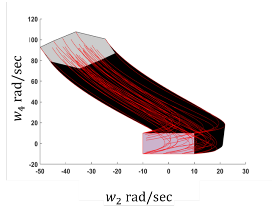
(b) CORA
