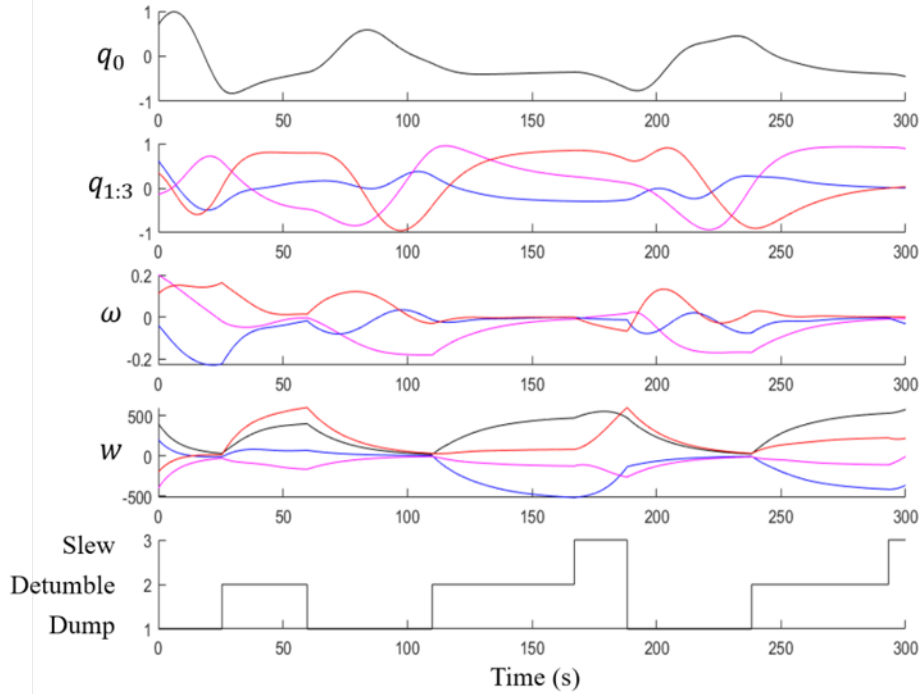
Fig. 4 For certain initial conditions found using falsification techniques, the spacecraft cycles between Dump, Detumble, and Slew without converging to Stablize.
