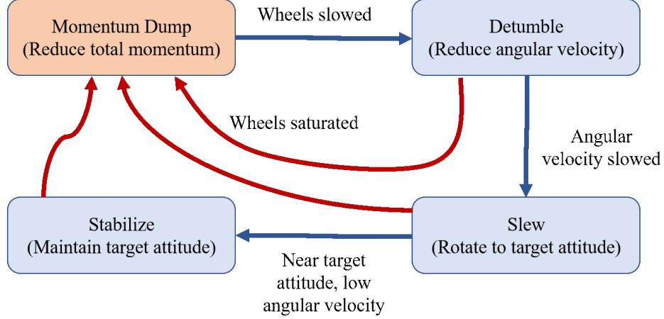
Fig. 1 Modes of the hybrid satellite benchmark.
