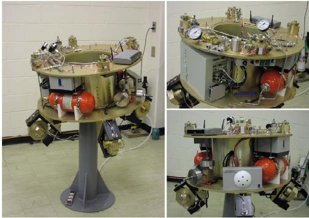
Fig. 2 The completed IACS spacecraft simulator.
