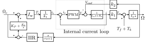
Fig. 13 Implementation of PI servo loop
