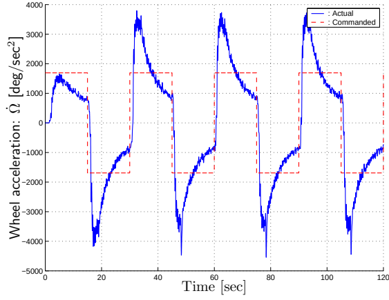
a) Wheel Acceleration \ddot{\Omega} .
