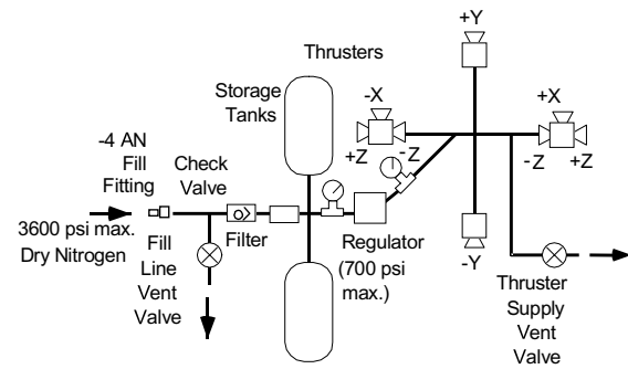
Fig. 3 Schematic of the thruster reaction control system (TRCS).
