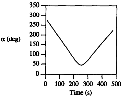
Fig. 10. Orientation angle (optimum mass trajectory).
