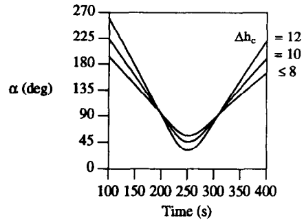
Fig. 6. Orientation angle (optimum force trajectories).
