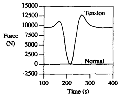
Fig. 5. Tension and normal forces on probe.
