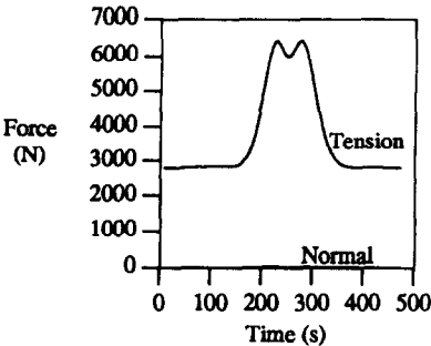
Fig. 12. Tether forces on the probe (optimum mass trajectory).
