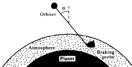
Fig. 1. Aerobraking tether.
