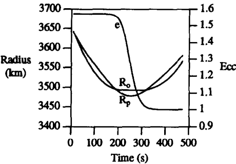
Fig. 11. End point positions and eccentricity (optimum mass trajectory).
