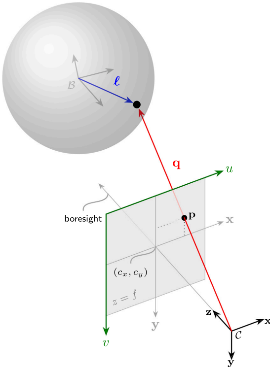
Fig. 2. Camera model geometry.
