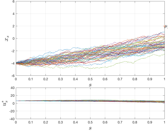
Fig. 2: The implementation of a naïve approach in attempting to reach the target via the terminal cost \frac{1}{2}(x_{t_f} - \mu_f)^2 .
