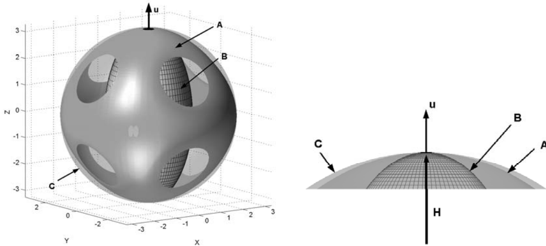
Figure 6. Inescapable singularity of VSCMG
