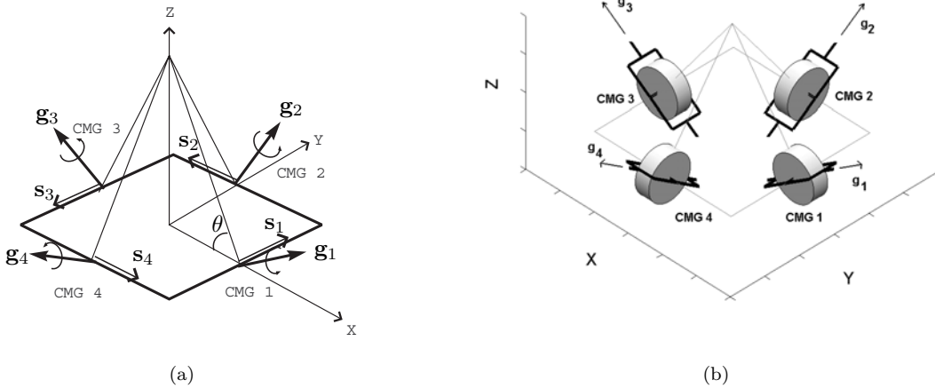
Figure 1. A VSCMG system with pyramid configuration
