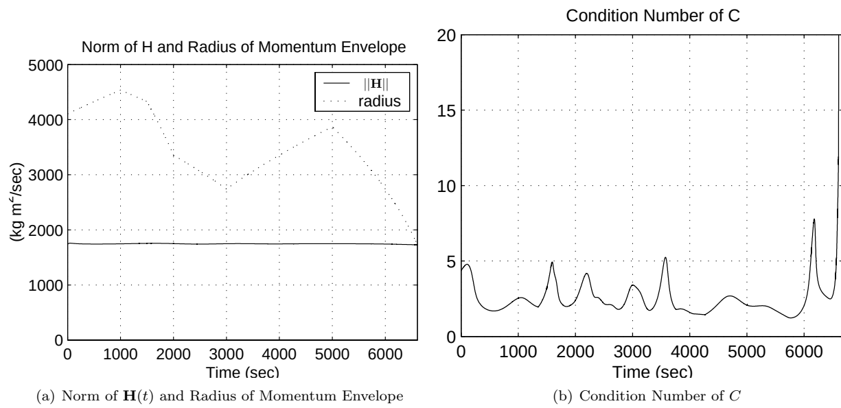
Figure 11. Inescapable Singularity
