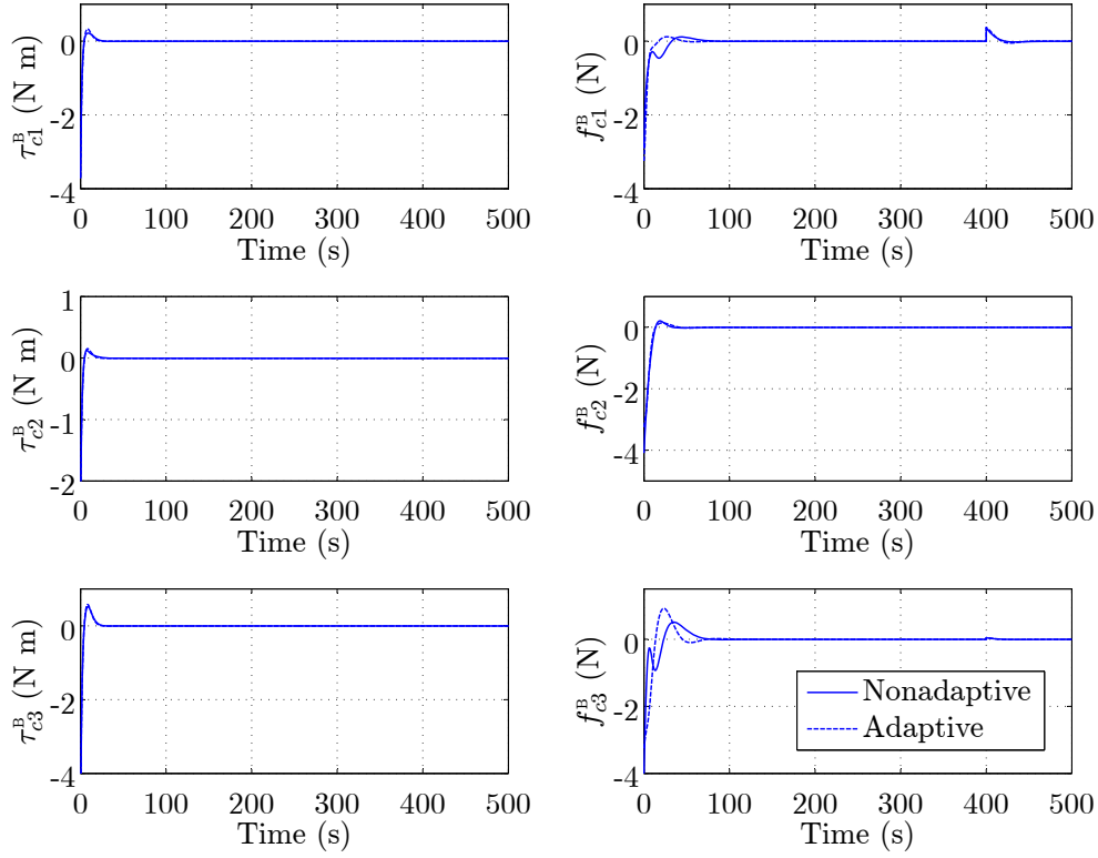
Figure 8. Control force and torque.
