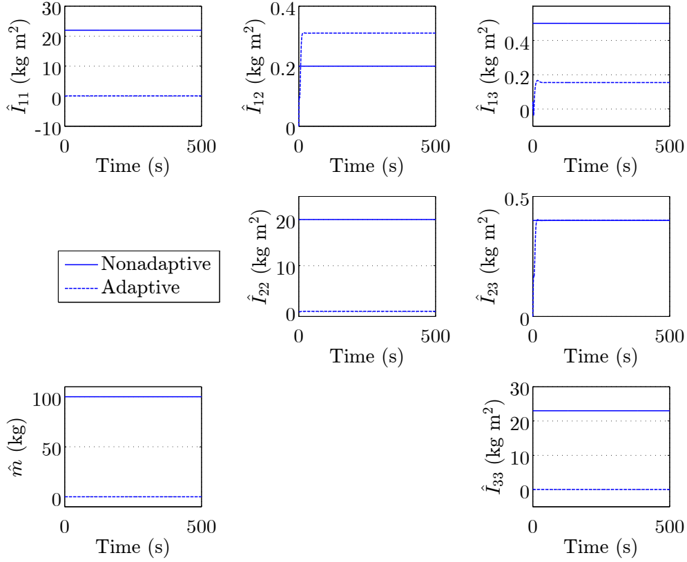
Figure 6. Mass and inertia matrix estimation for low-exciting reference motion.
