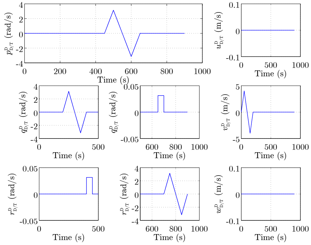
Figure 9. Reference motion for identification.
