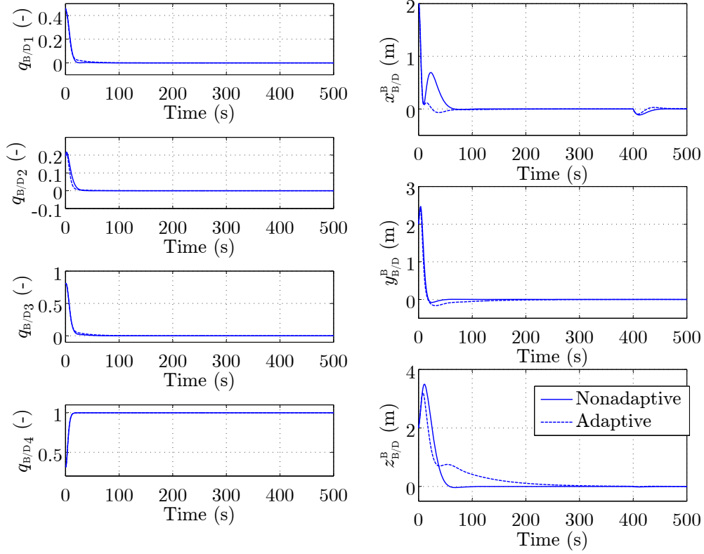
Figure 4. Relative attitude and position expressed in the body frame.
