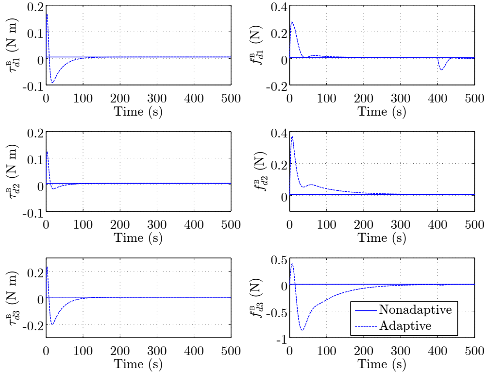
Figure 7. Dual disturbance force estimation.
