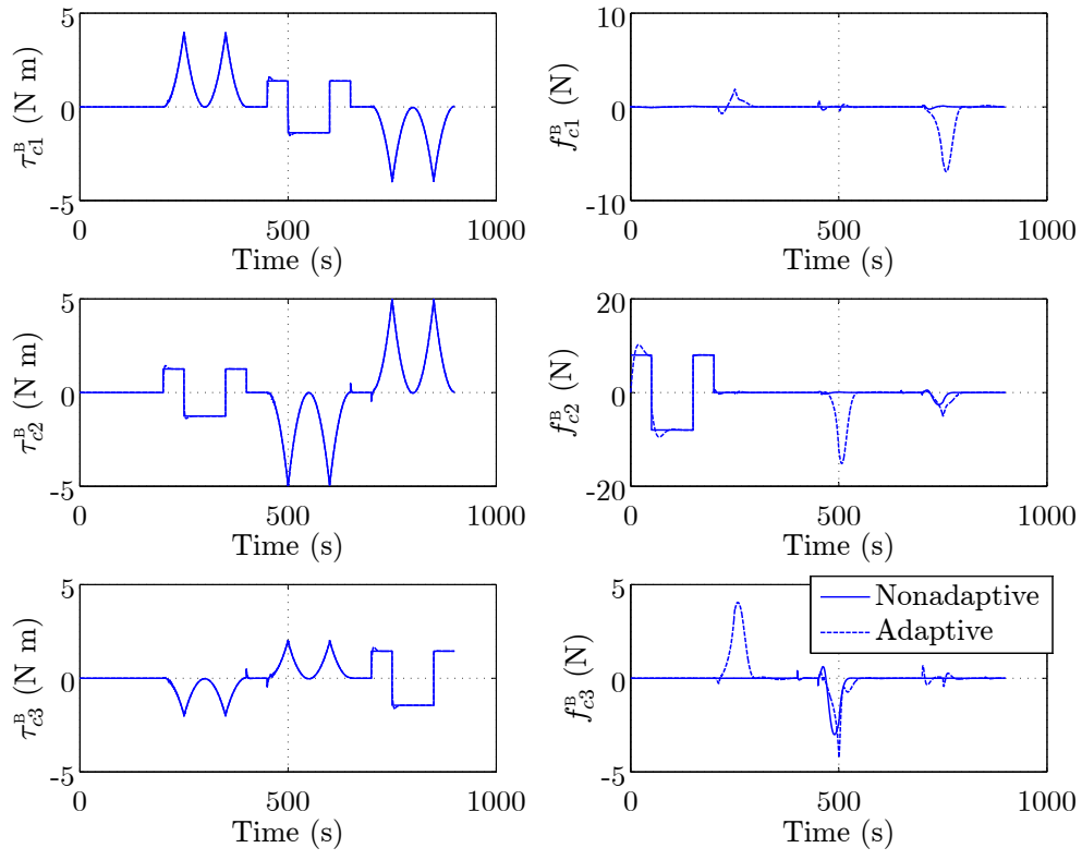
Figure 11. Control force and torque during identification.
