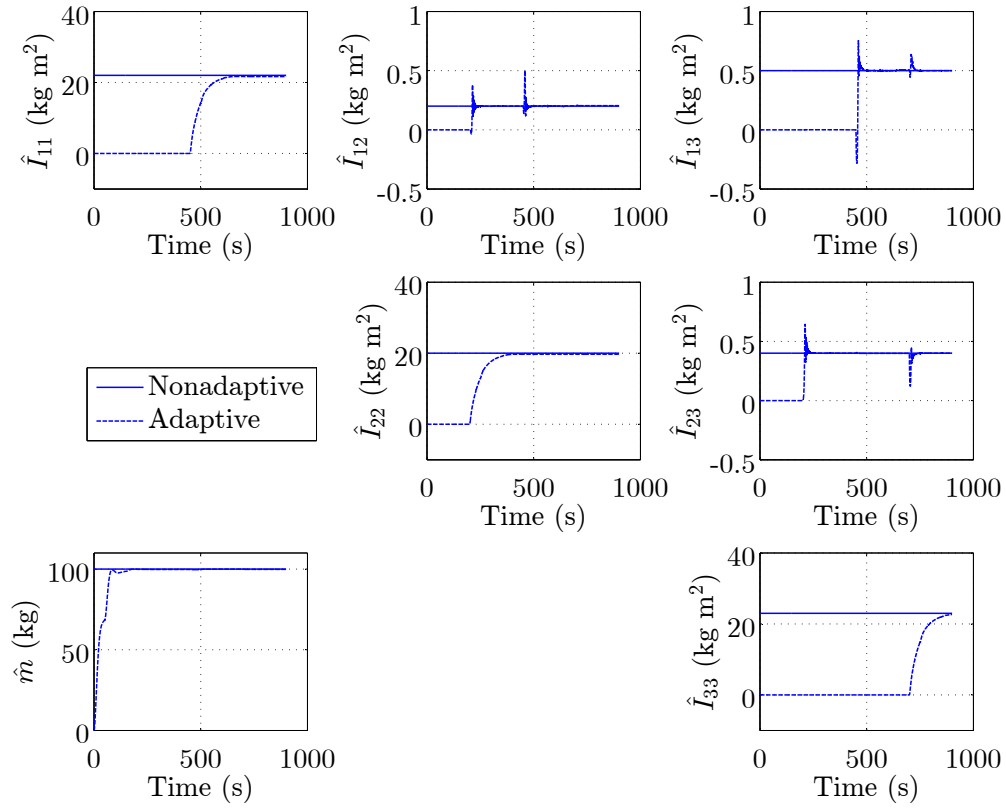
Figure 10. Mass and inertia matrix identification.
