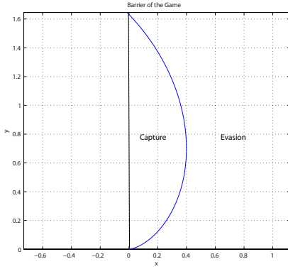
Fig. 3. The barrier, given by equations (31) and (31) for v_e = v_p = 1 and R = 0.7 , for the case in which the pursuer appears in the upper right quadrant. By virtue of symmetry, a reflection on the y -axis will provide the barrier for the case in which the pursuer is located at the upper left quadrant.
