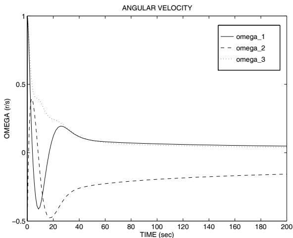
Figure 1: Angular velocity history.
